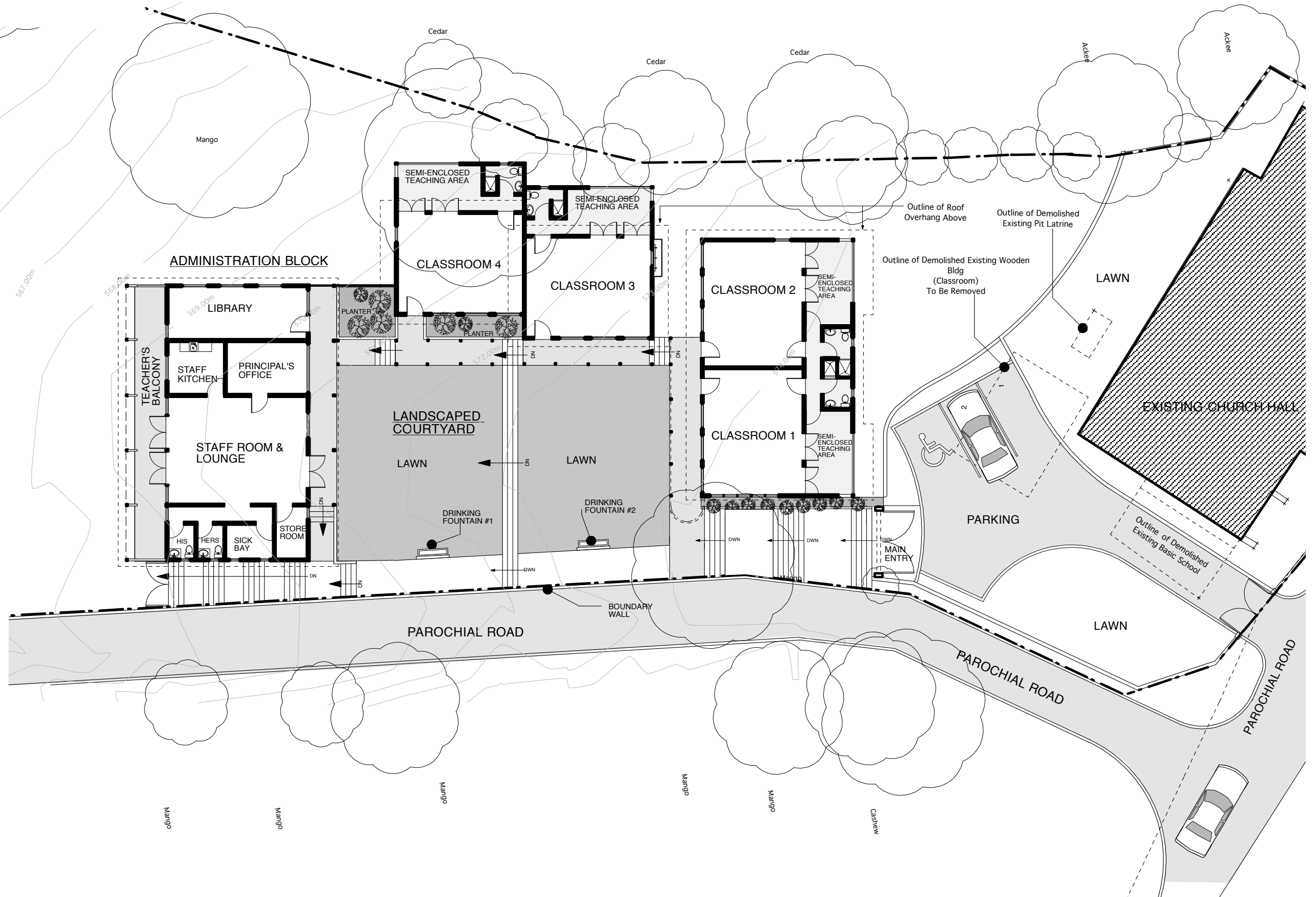
entry level floor plan
